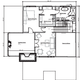
Upper Level
